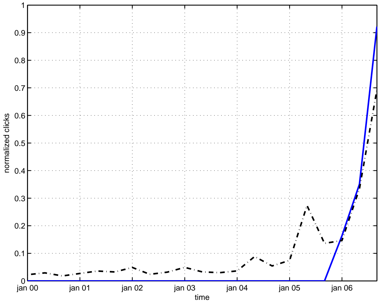
effect finite size
