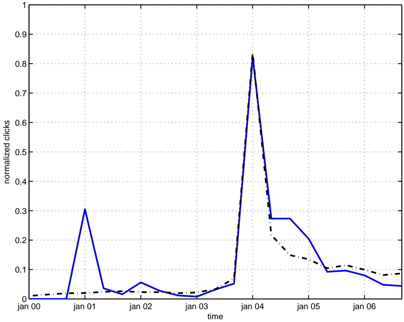
e(n) algebra
