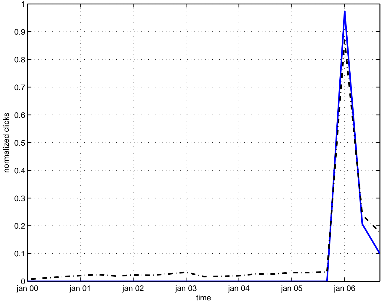
e(8) x so(8) gauge field theory
