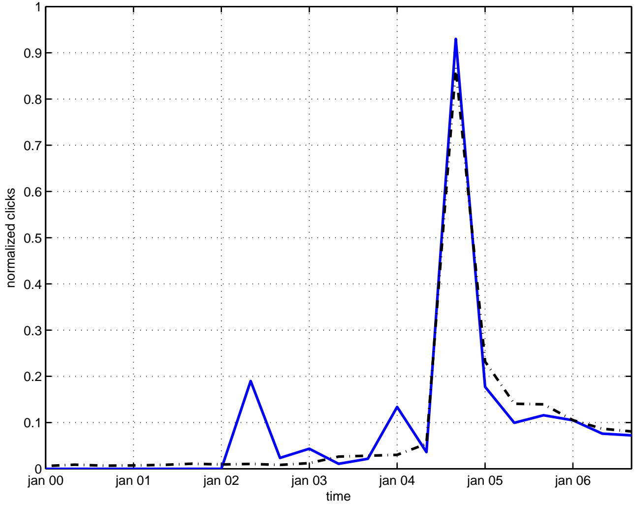
e(8) symmetry
