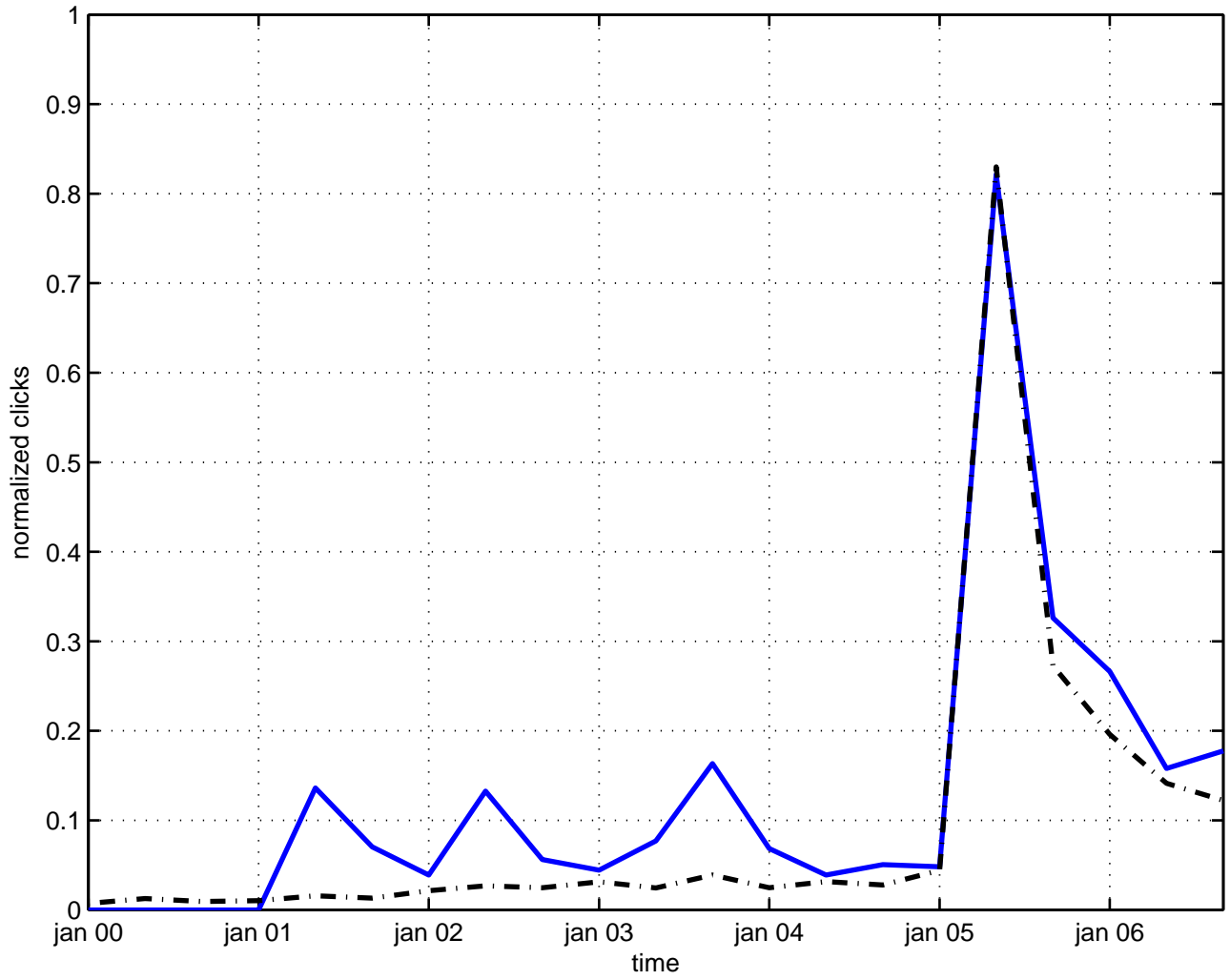
e(8) group theory
