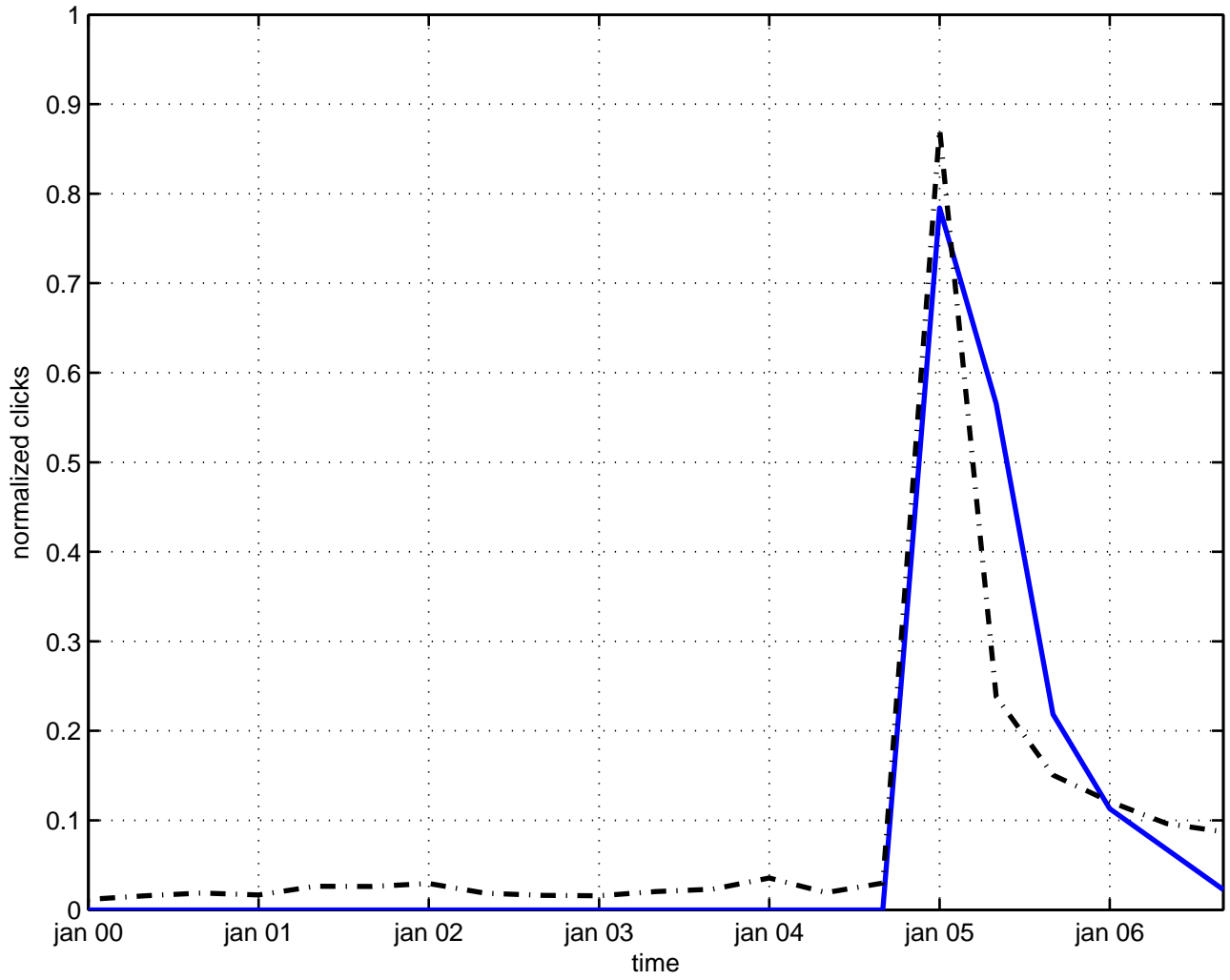
e(7) invariance
