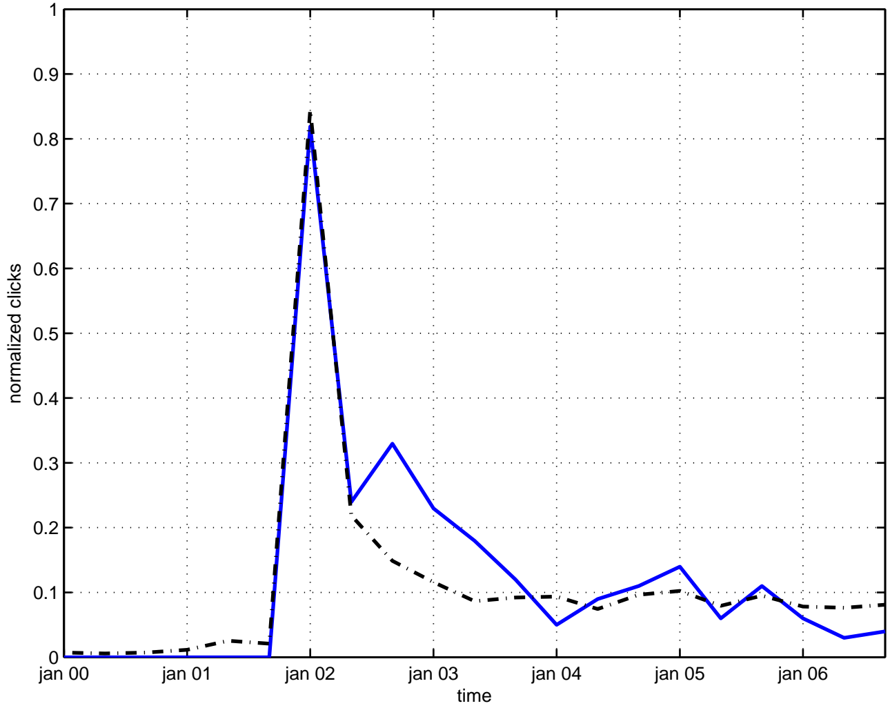
e(7) embedding
