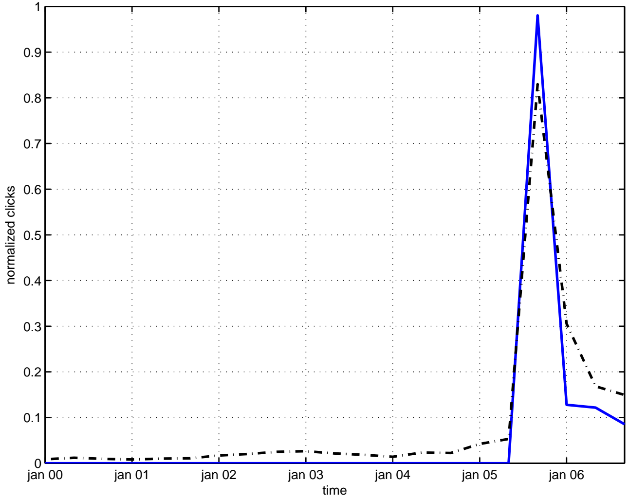
e(6) matrix model
