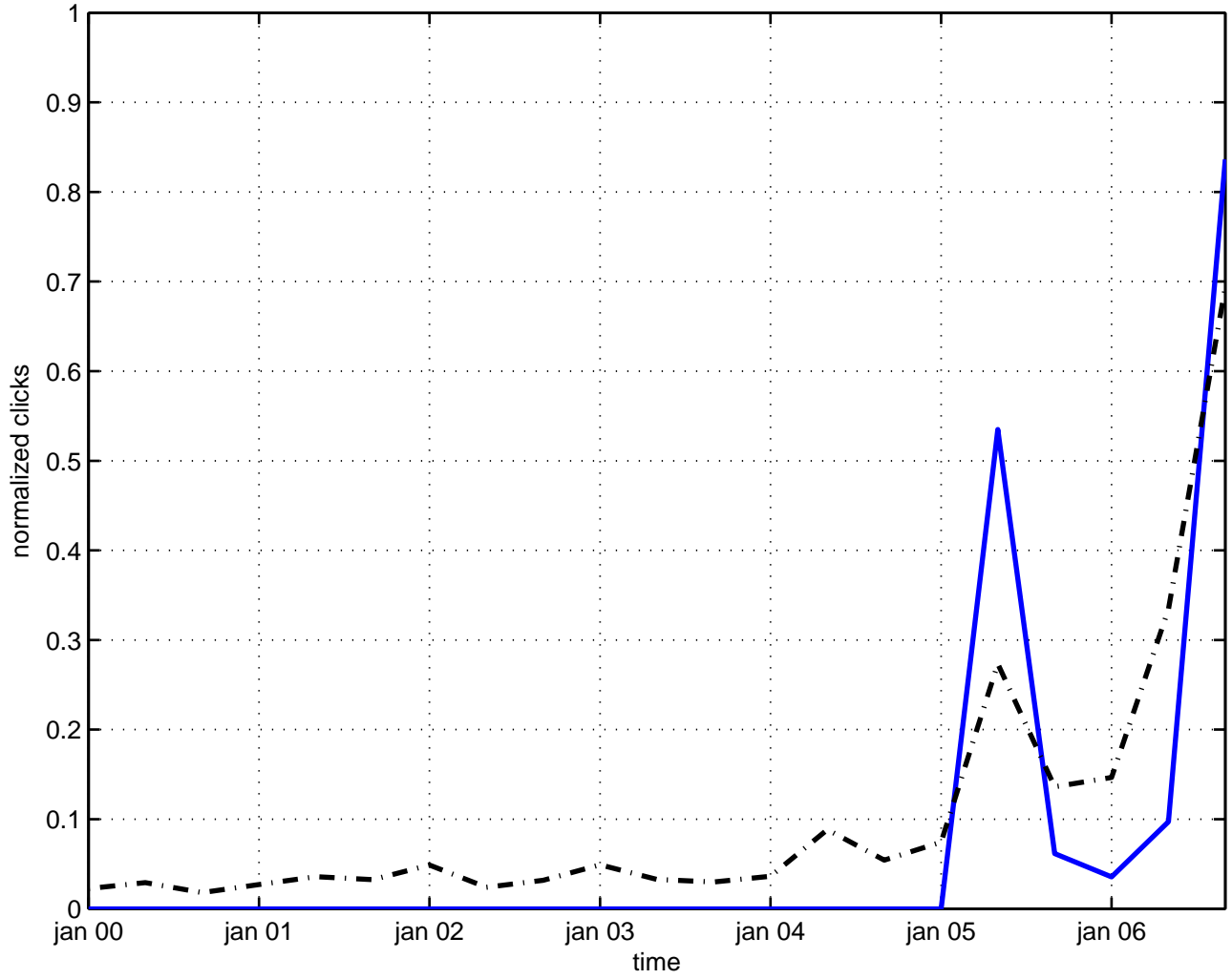
e(6) grand unified theory
