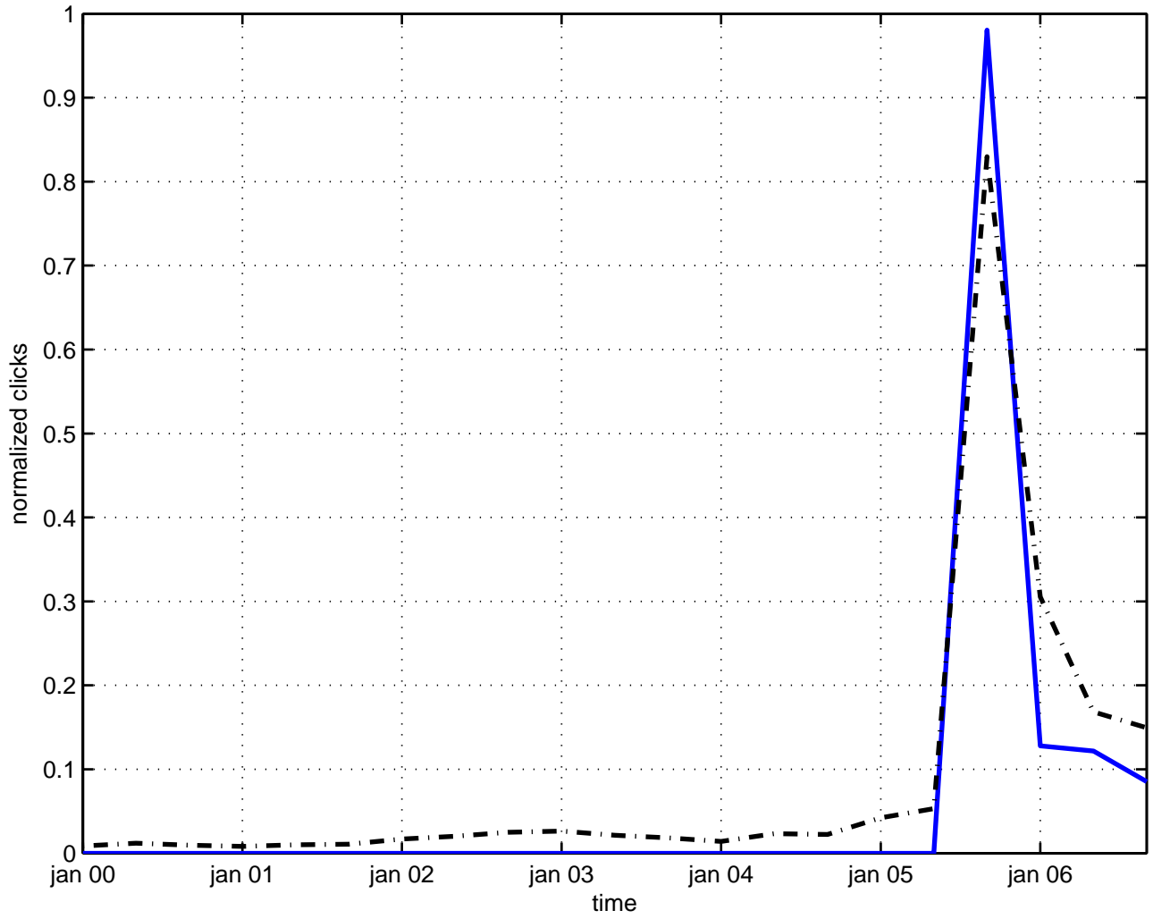
e(6) gauge field theory
