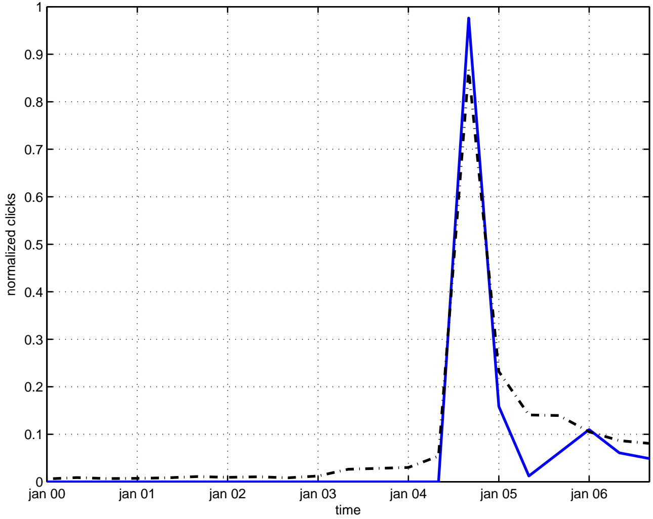
e(2) invariance
