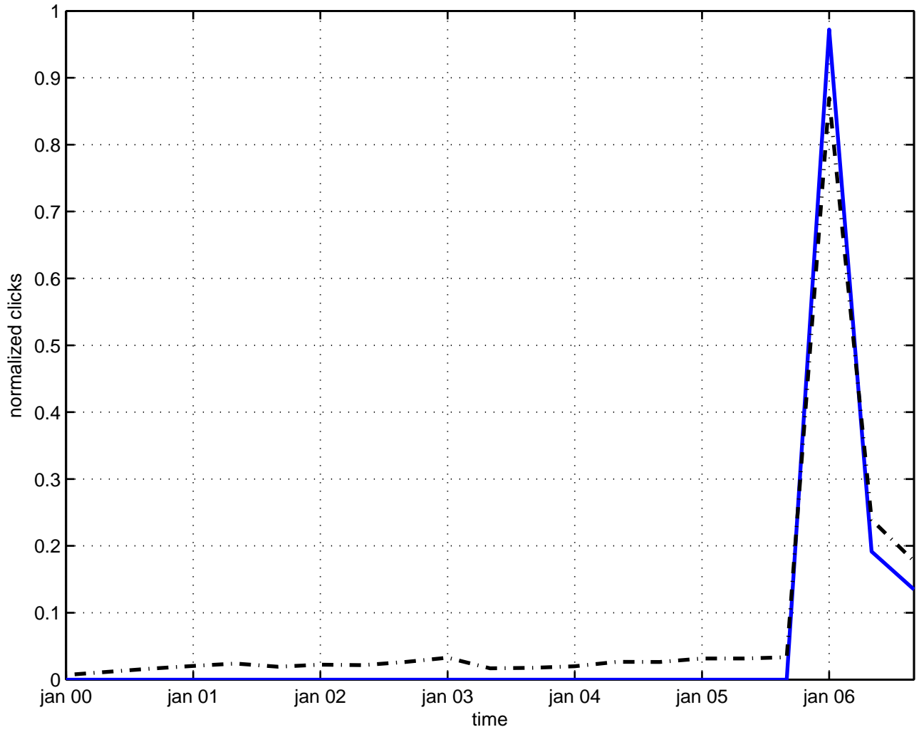
e(19) group theory
