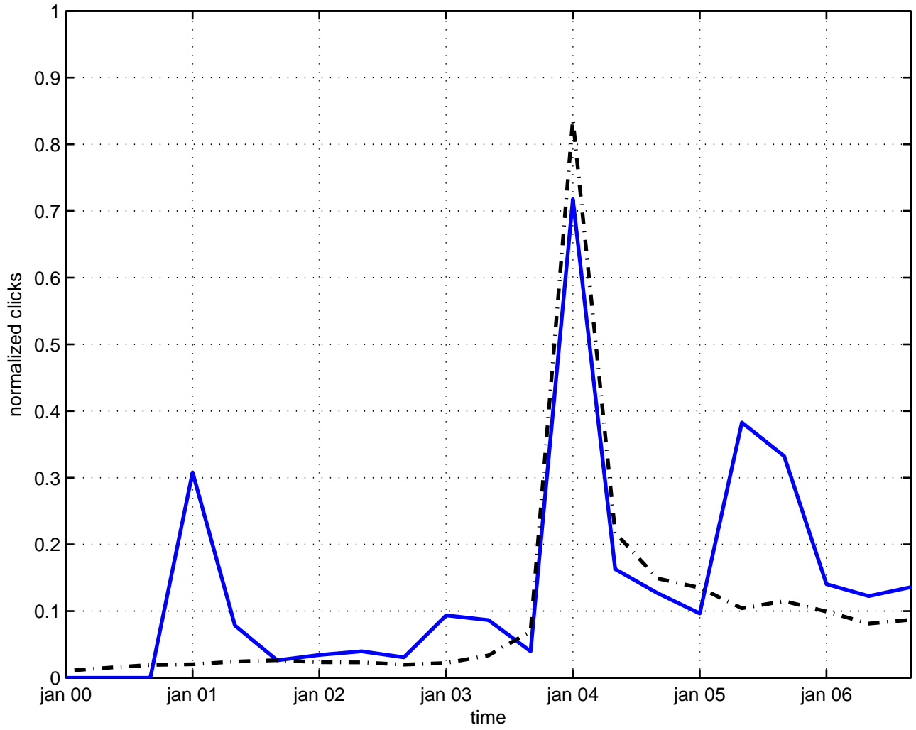
e(11) group theory
