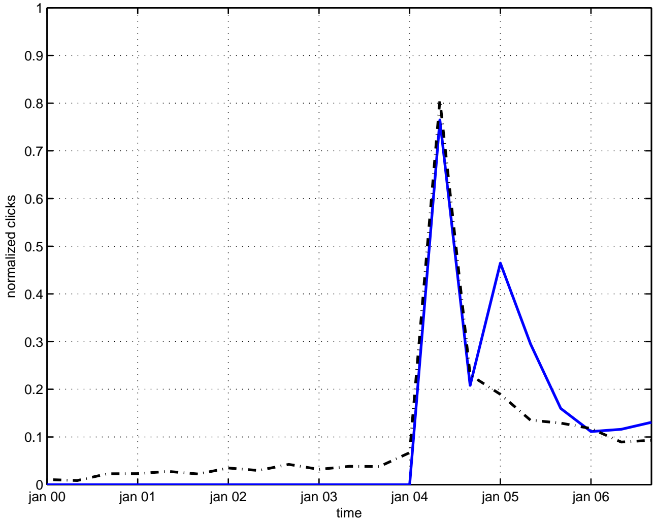
e(10) symmetry
