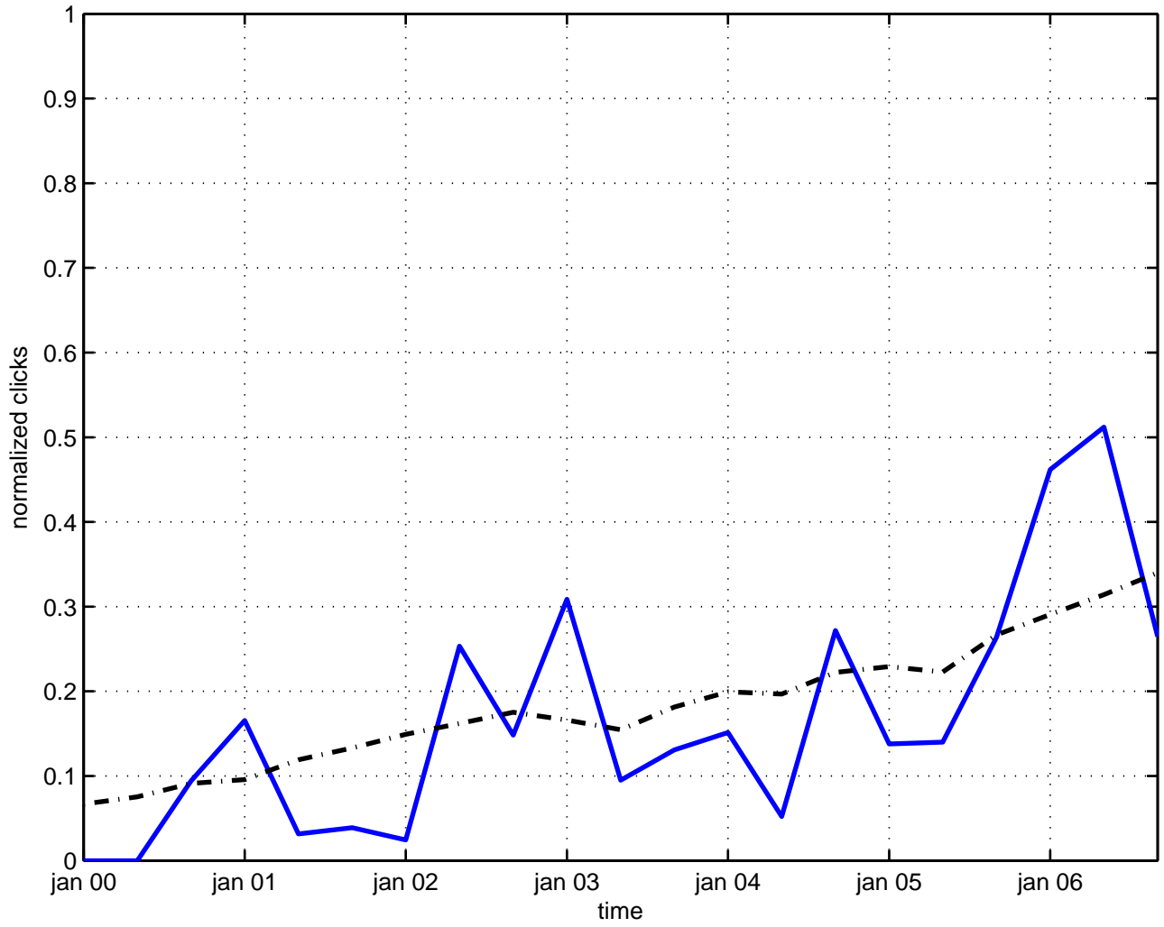
e(10) algebra
