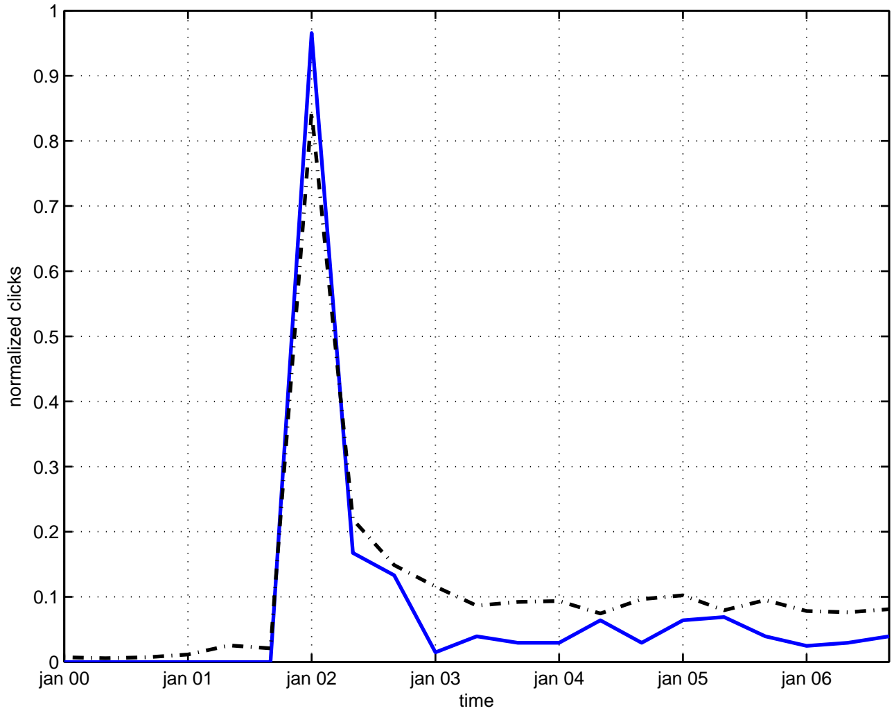
e(0) gauge field theory
