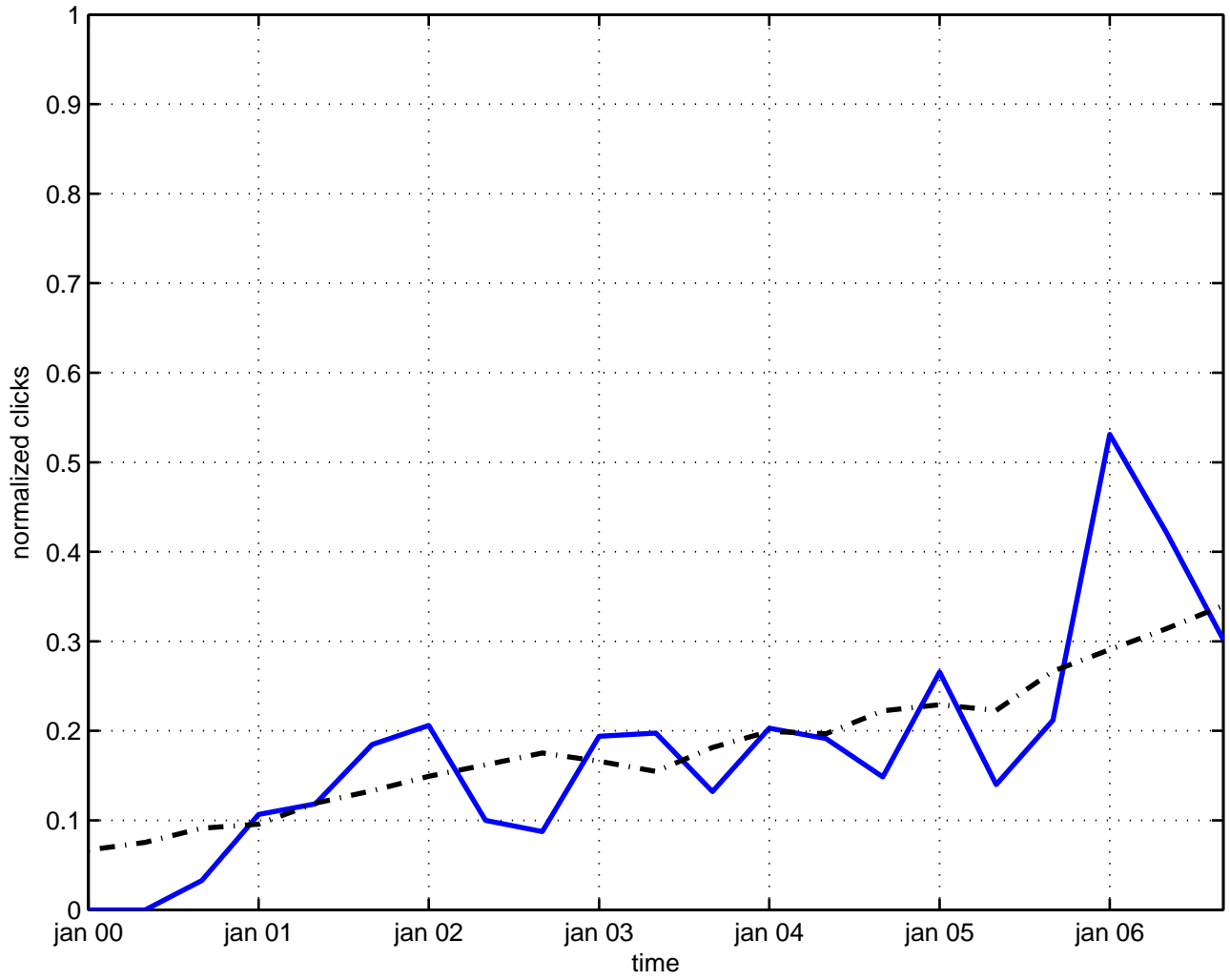
dynamical system
