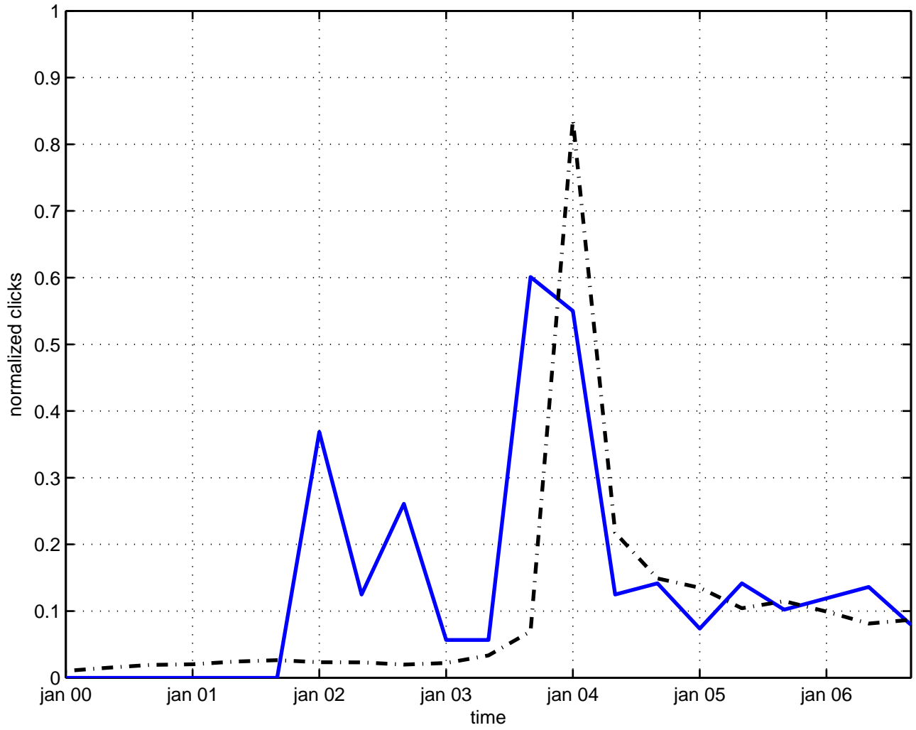
dynamical symmetry
