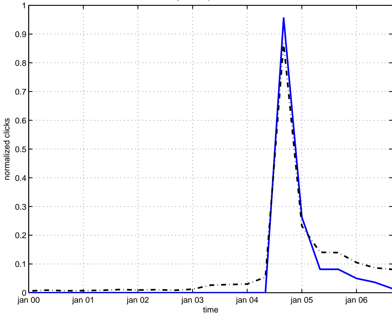
dynamic quantization
