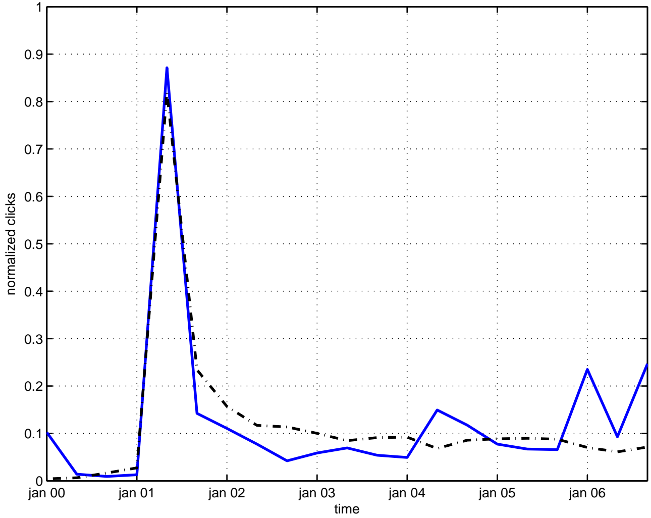
duality supergravity
