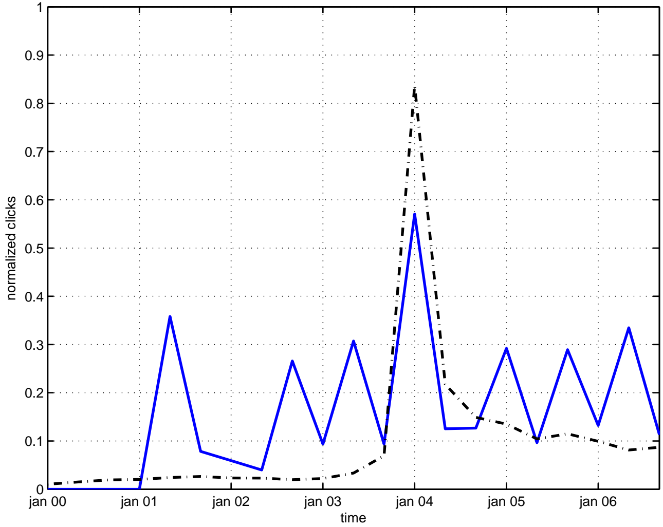
duality superconductivity
