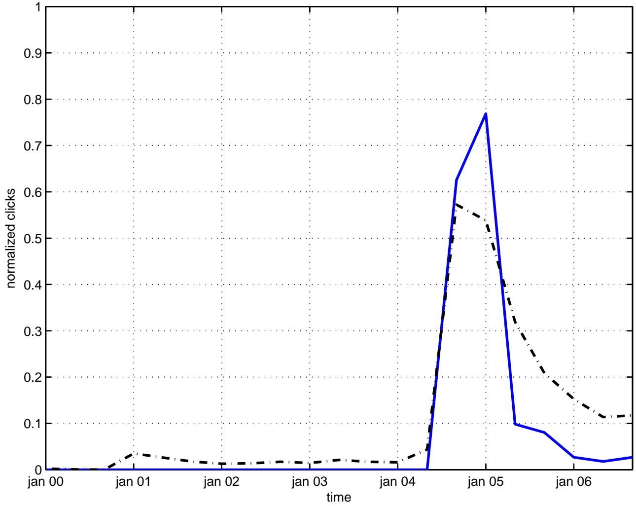
duality quark
