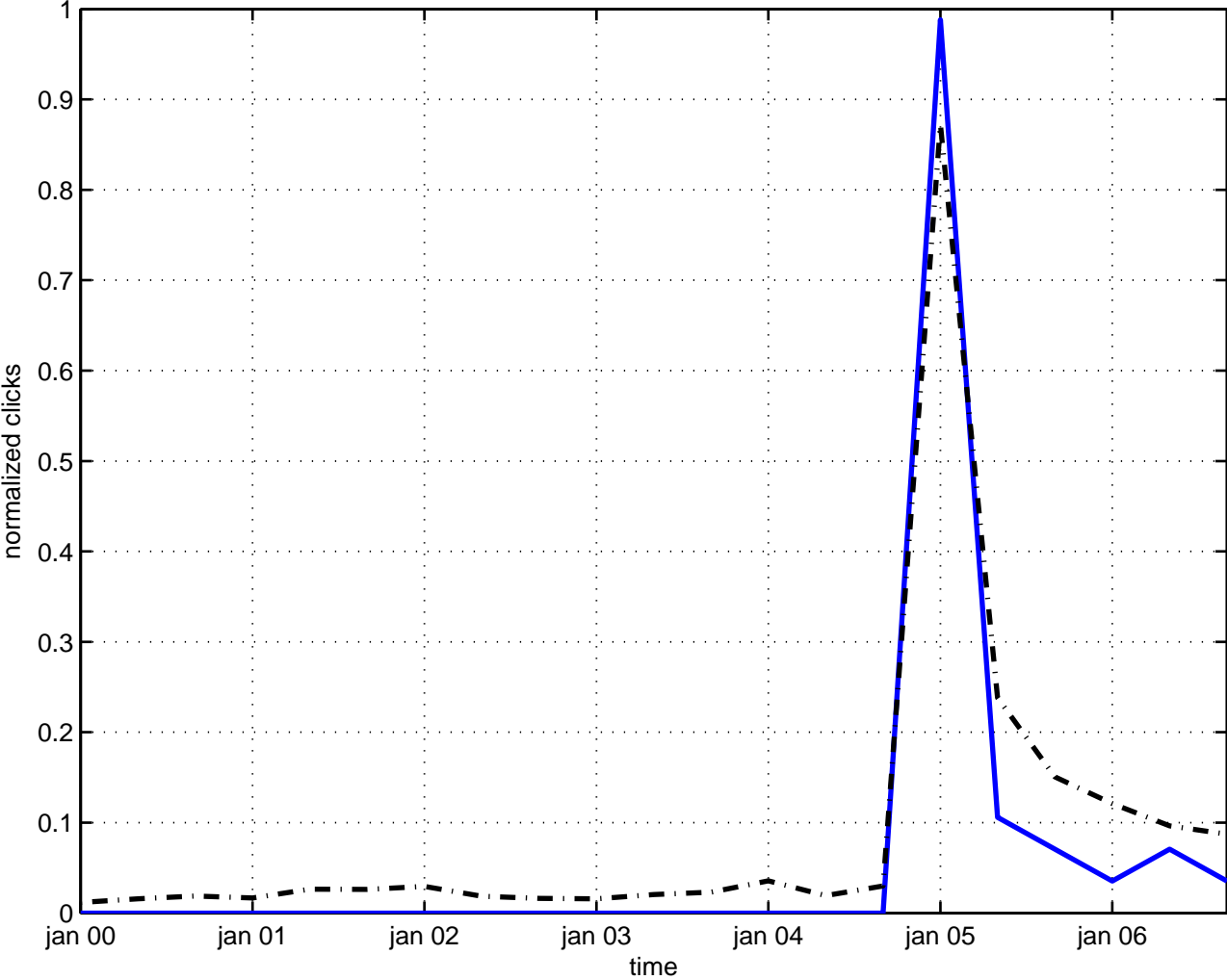
duality quantum chromodynamics
