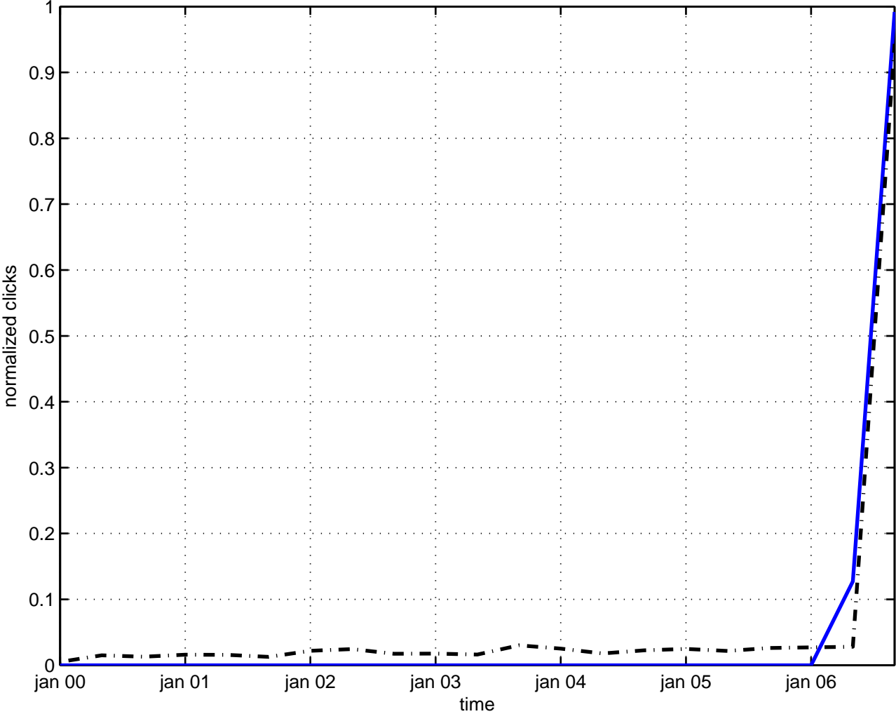
duality path integral
