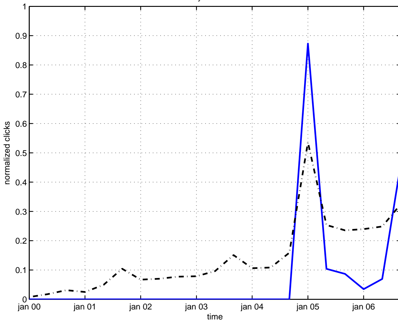
duality matrix model
