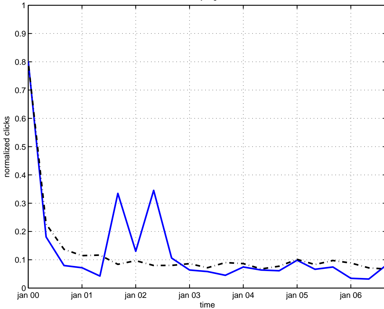
duality algebra
