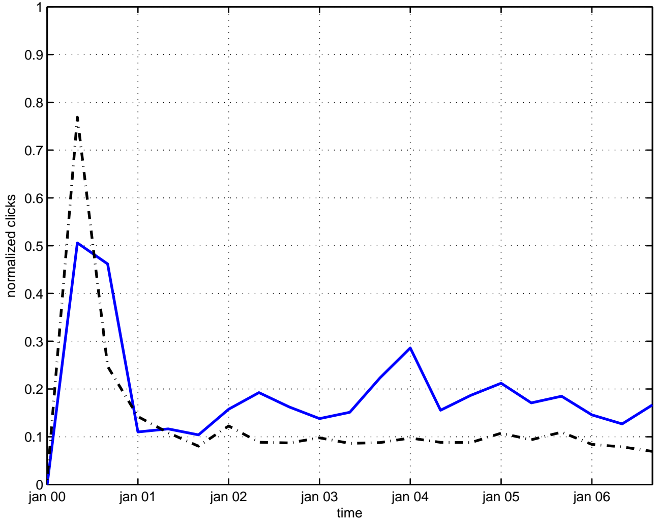
dual resonance model
