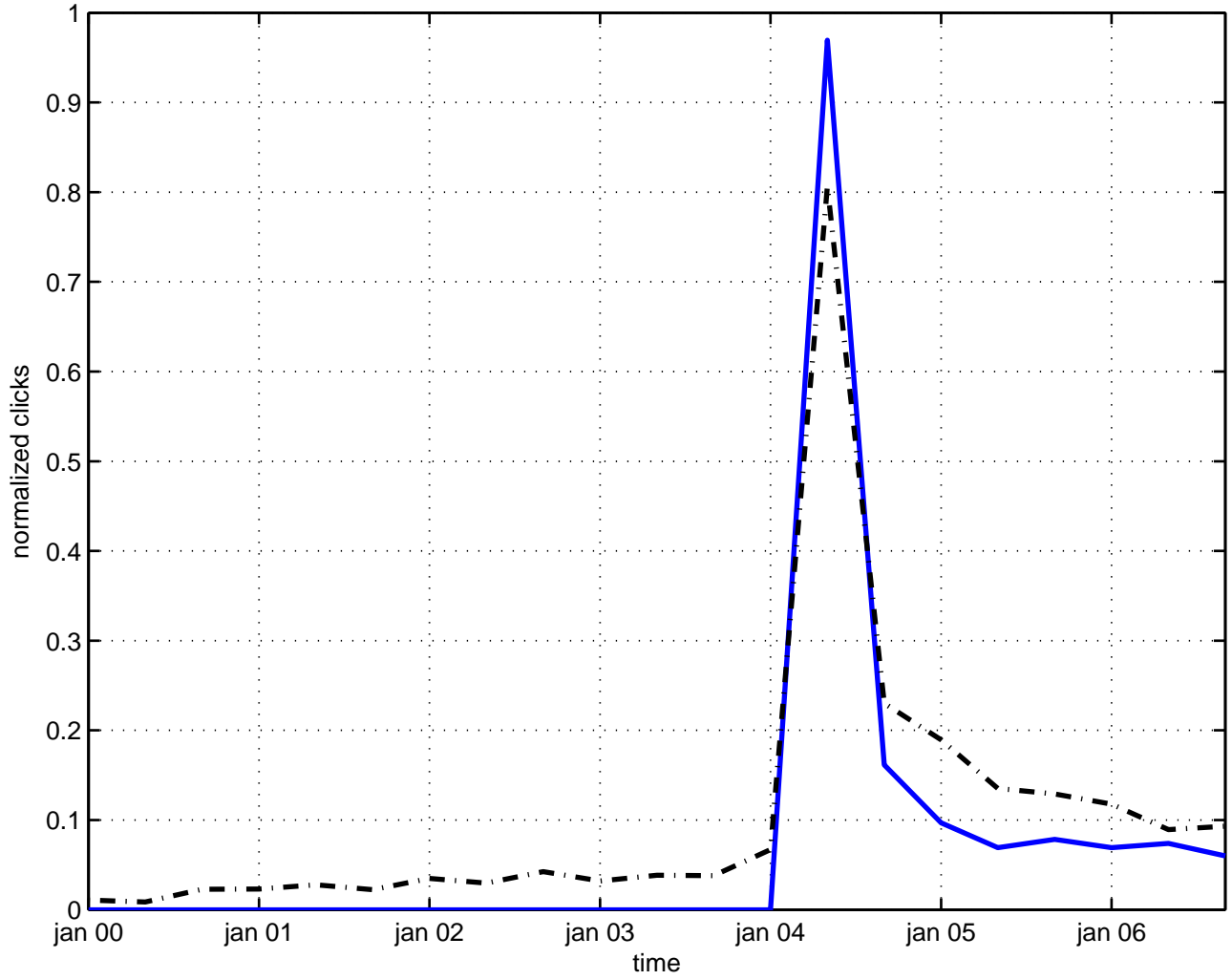
double relativity theory
