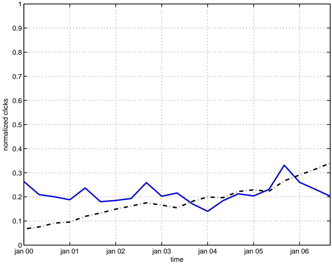
domain wall
