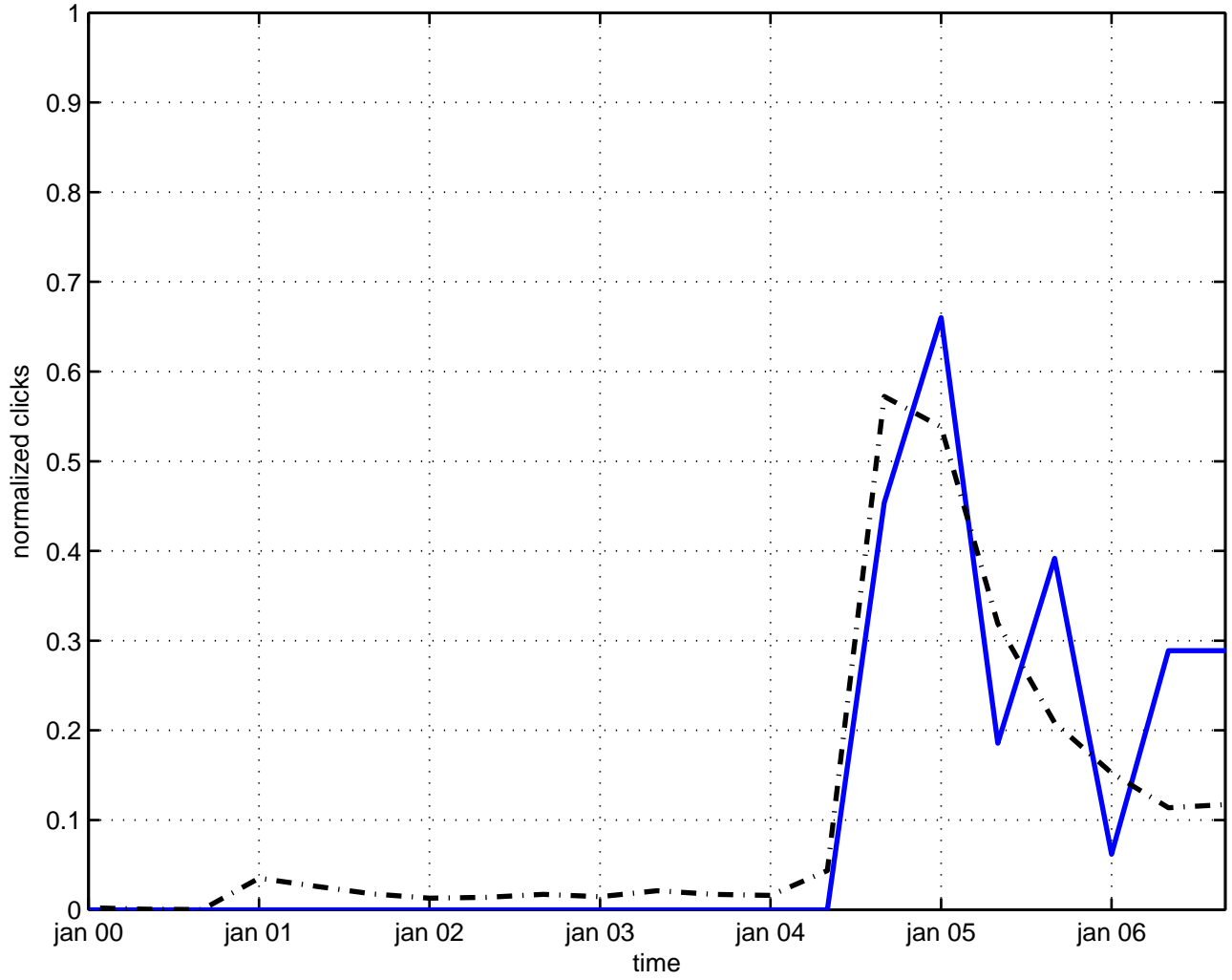
dissipation soliton
