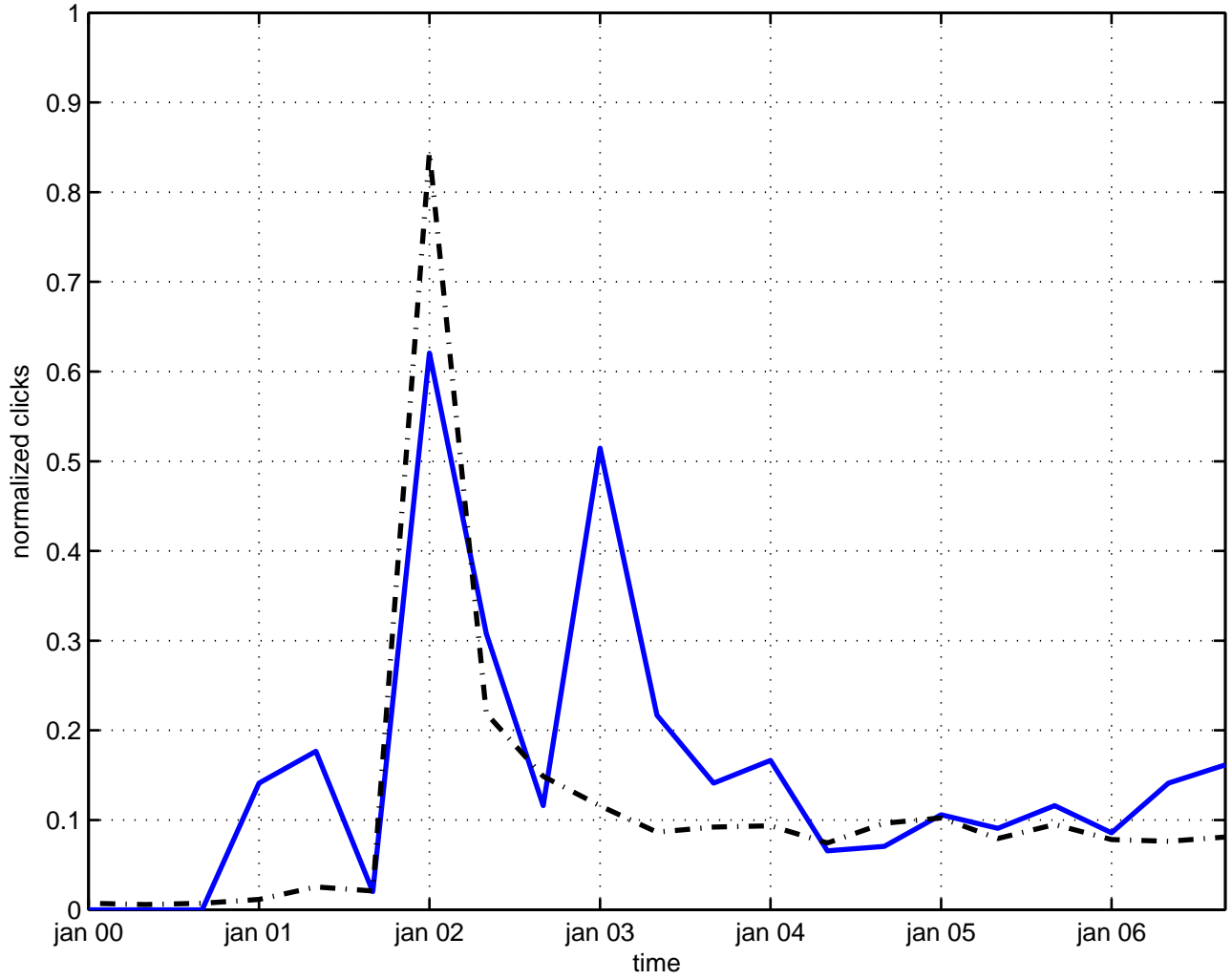
dissipation fluctuation
