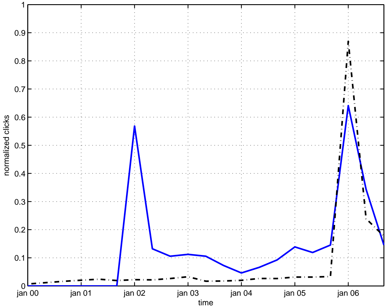
discrete transformation
