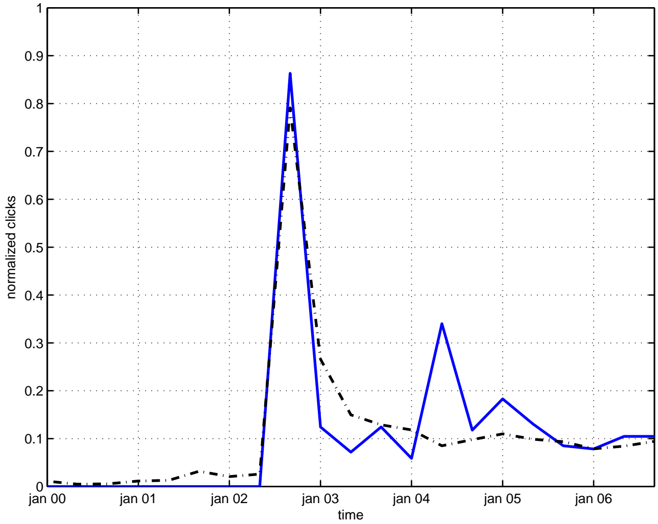
discrete topology
