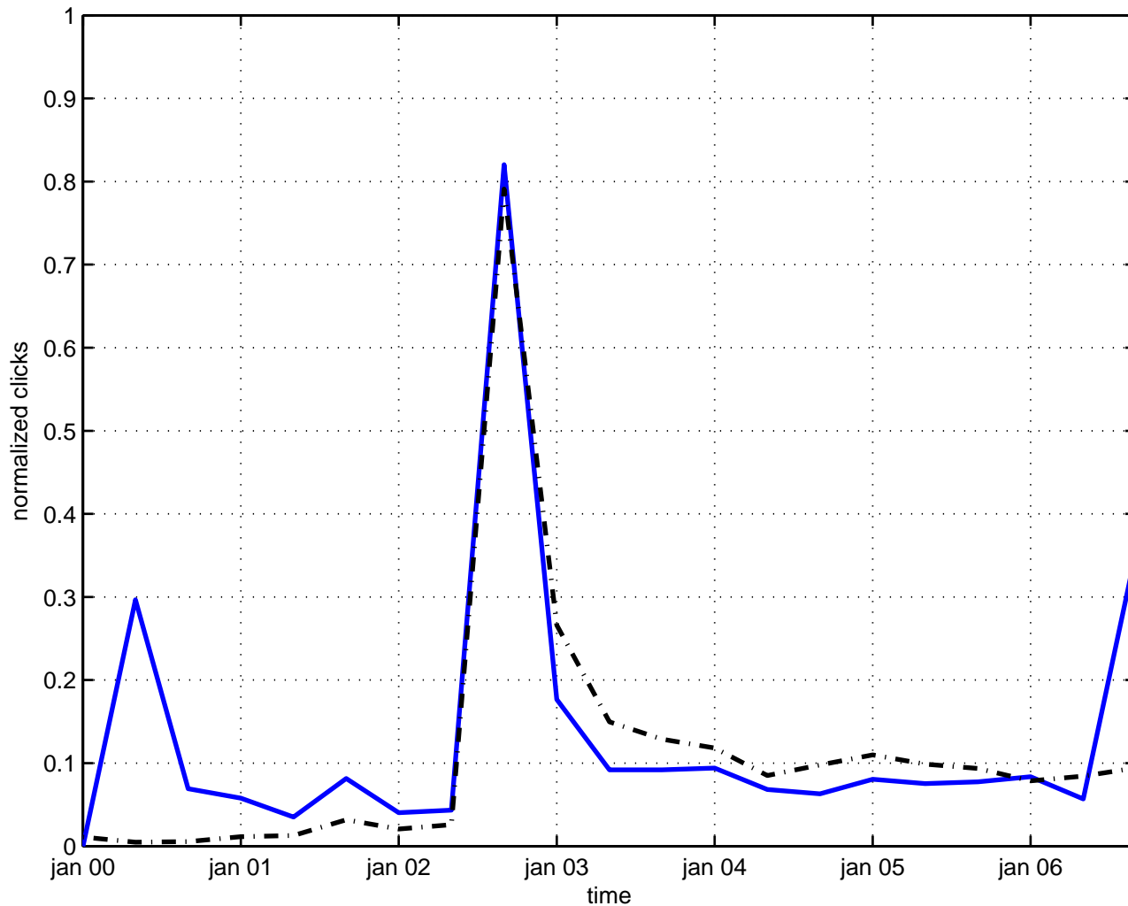
discrete time
