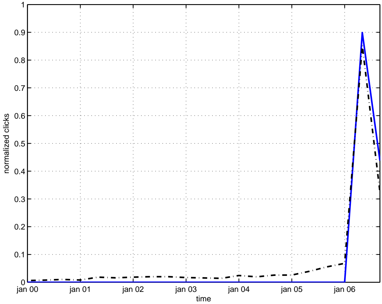
discrete symmetry breaking
