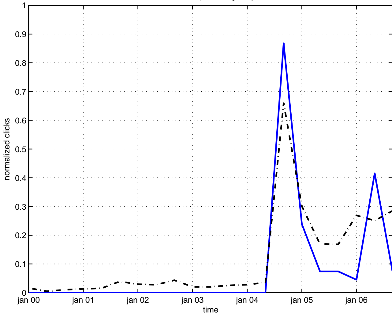
discrete quantum gravity
