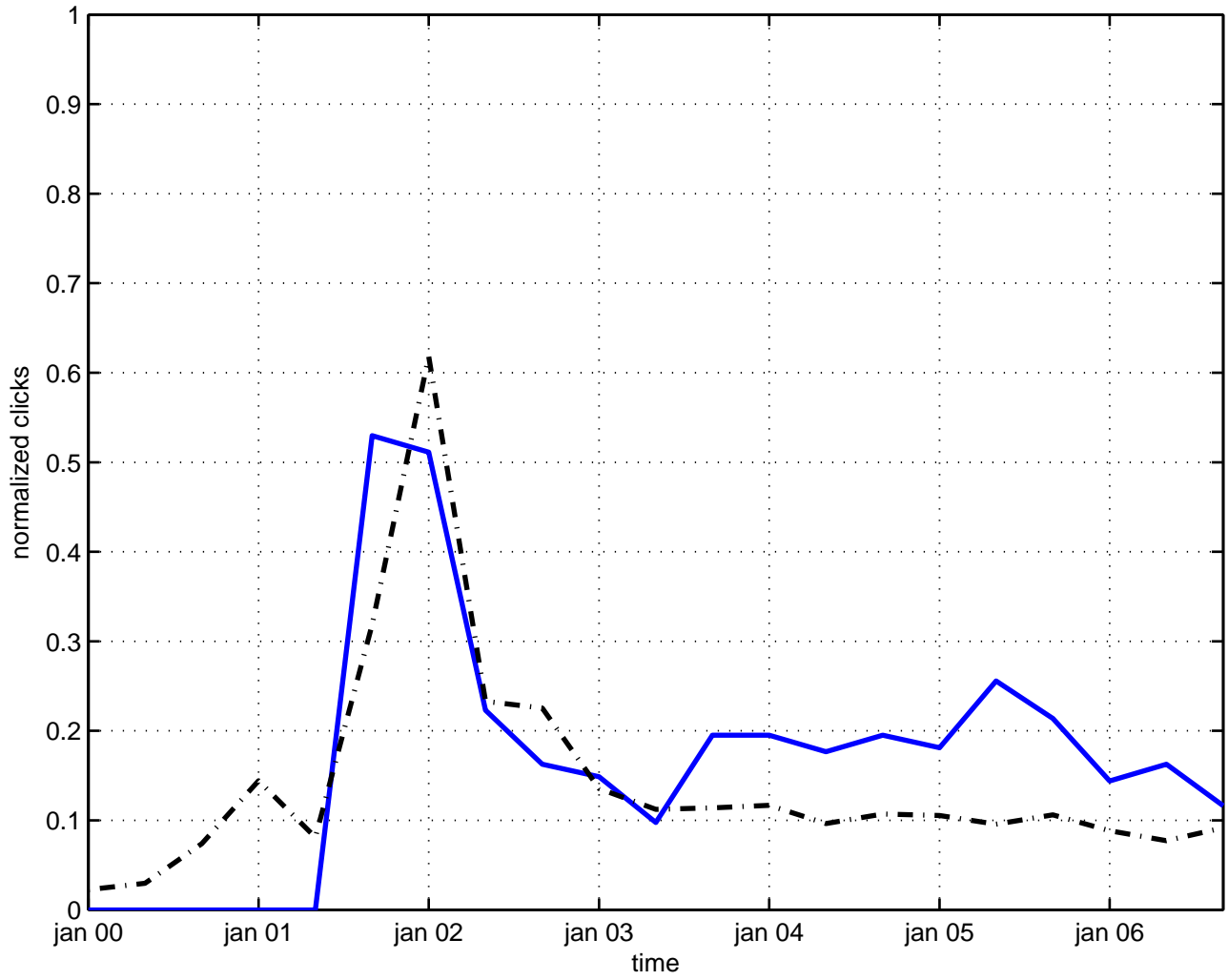
discrete mechanics
