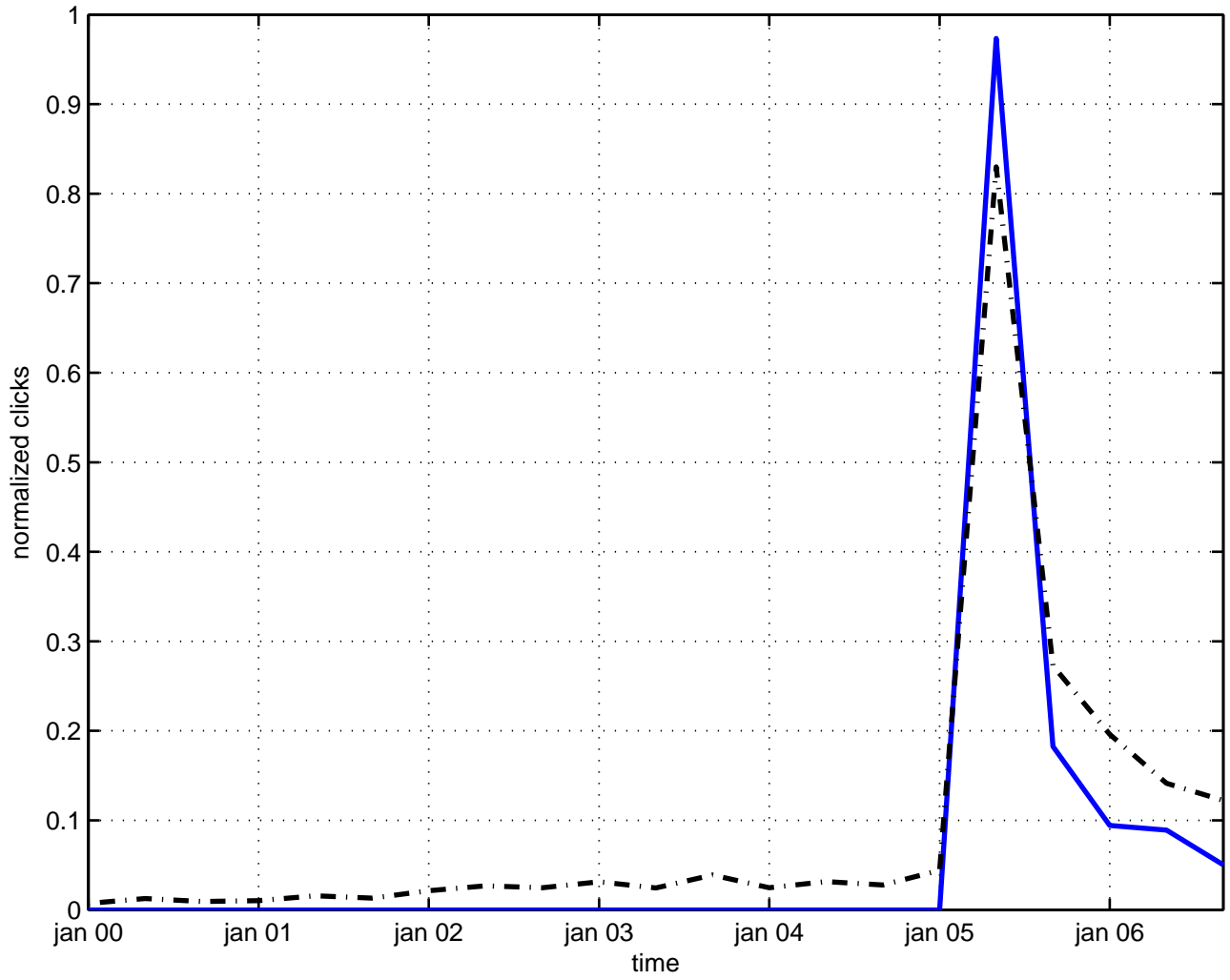
discrete hilbert space
