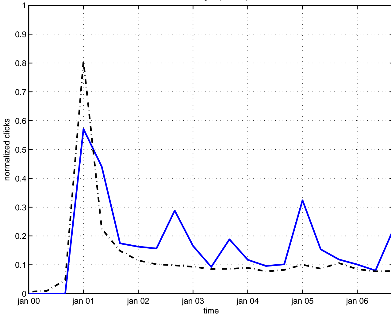
discrete group theory
