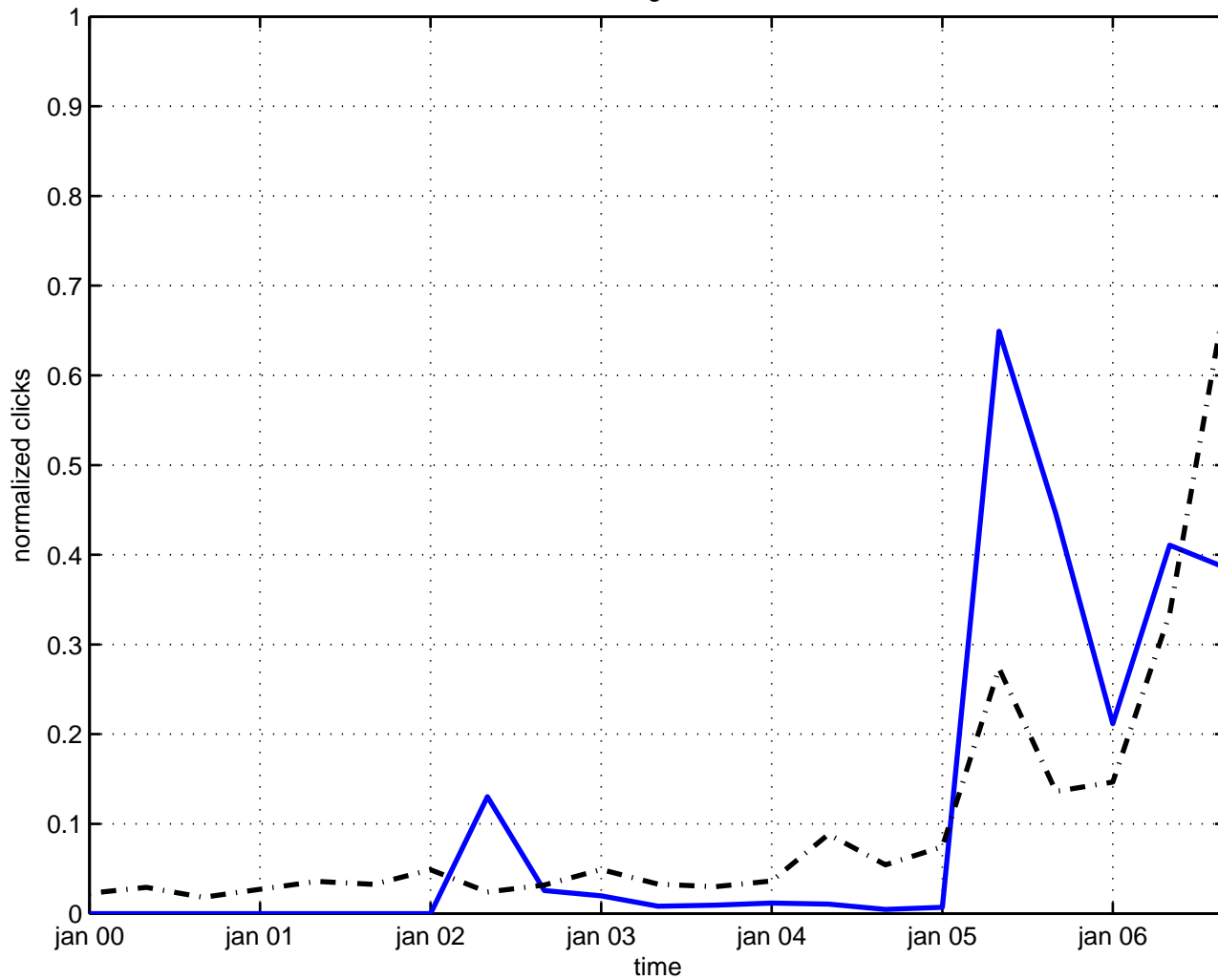
discrete gravitation
