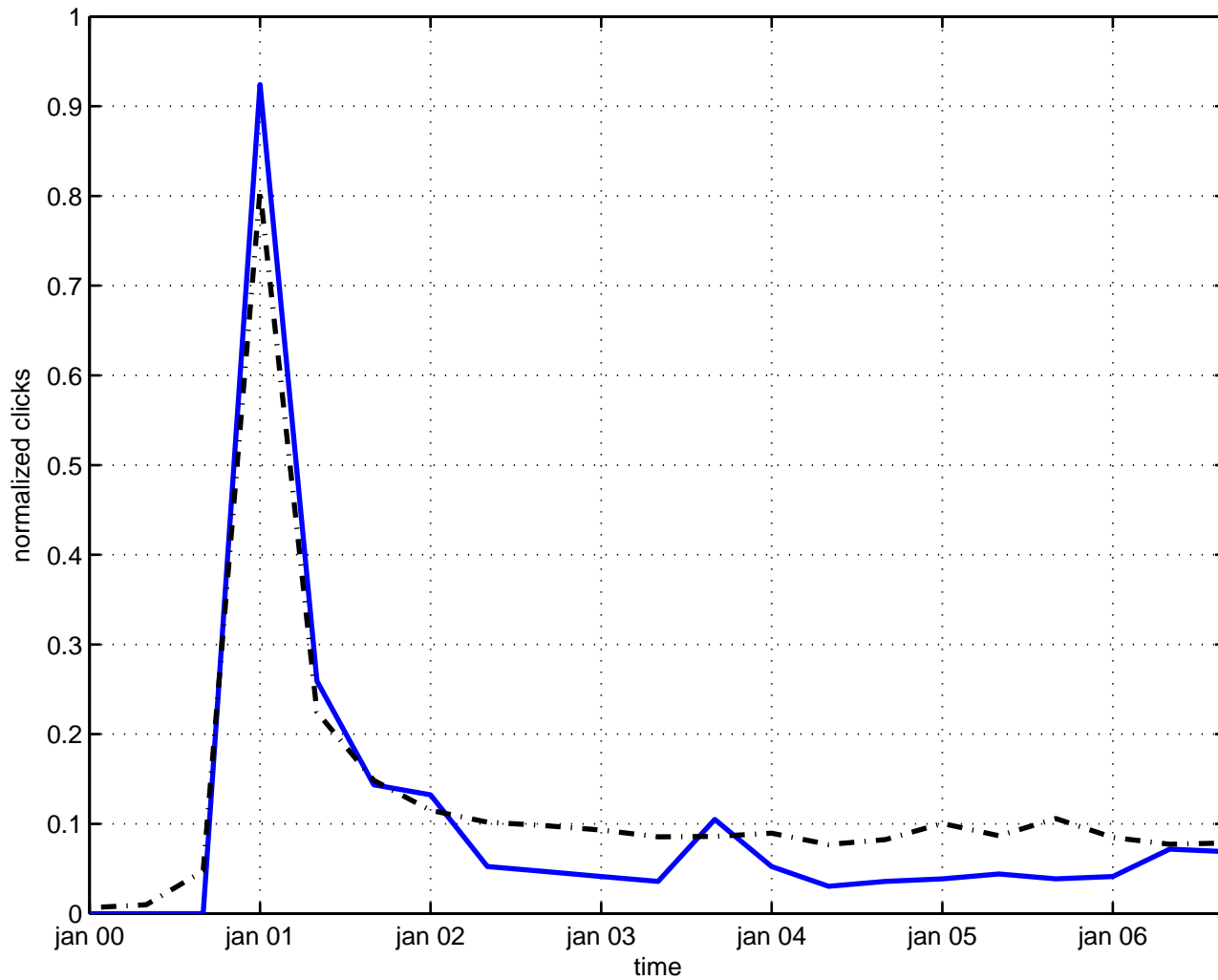
discrete flux
