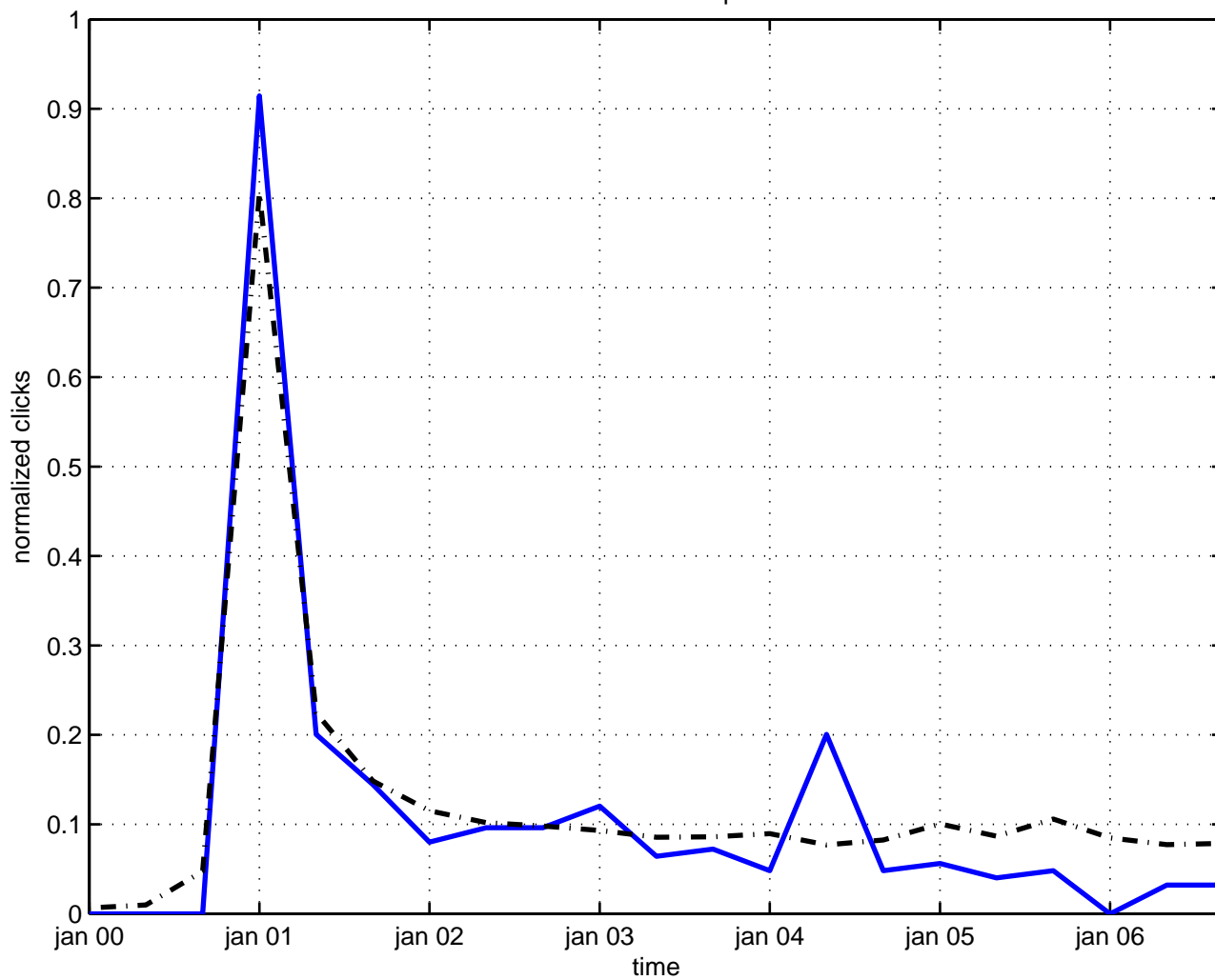
discrete diffeomorphism
