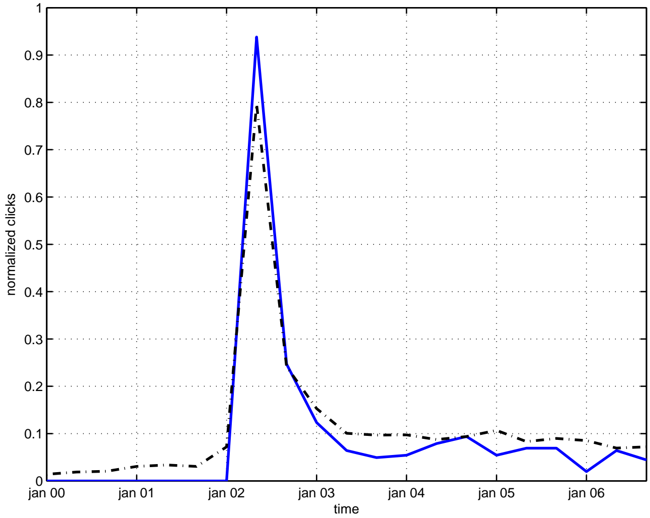
dirac zero mode
