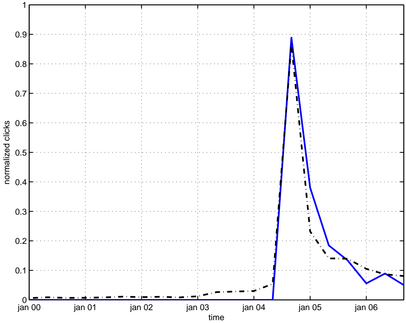
dirac perturbation
