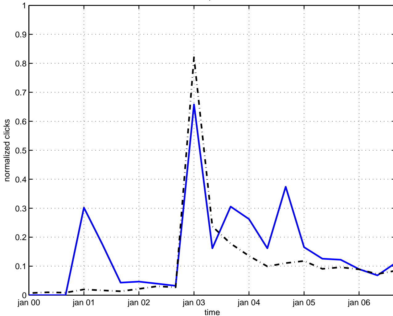
dirac particle
