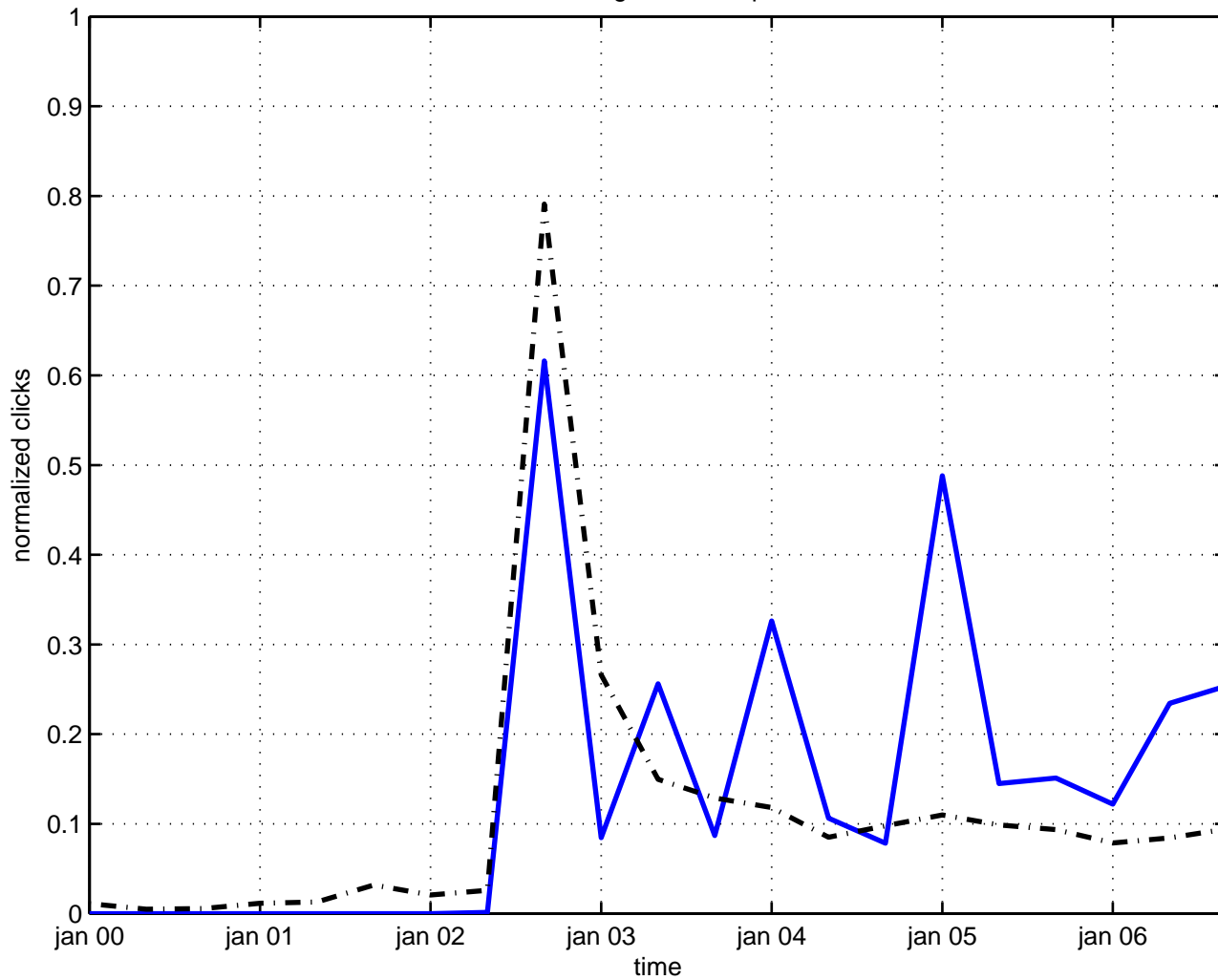
dirac magnetic monopole
