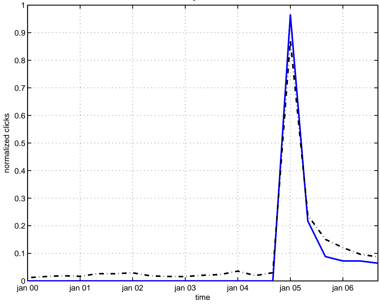
dirac magnetic moment
