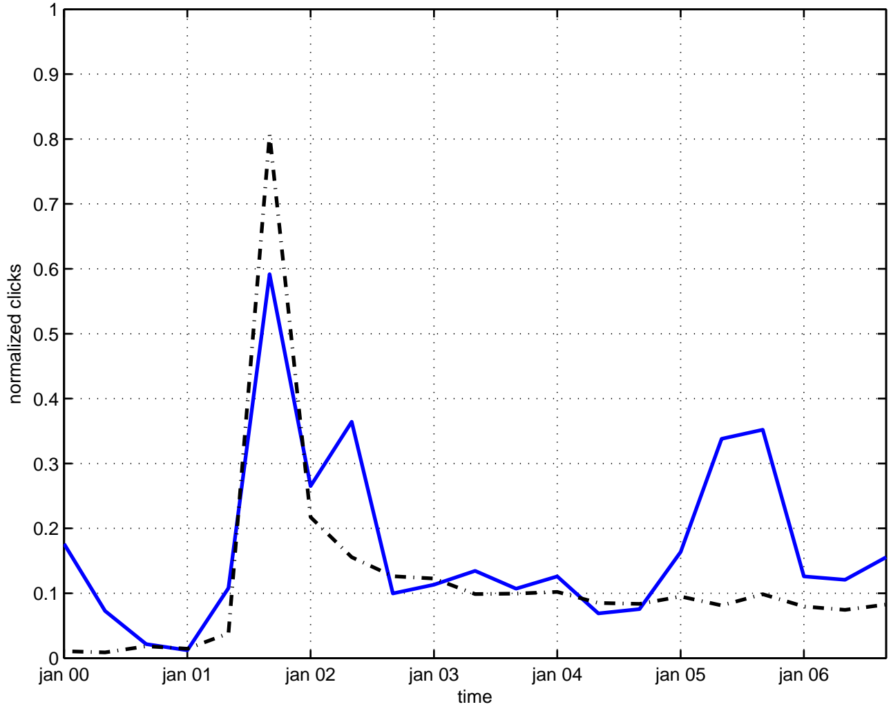
dirac field theory
