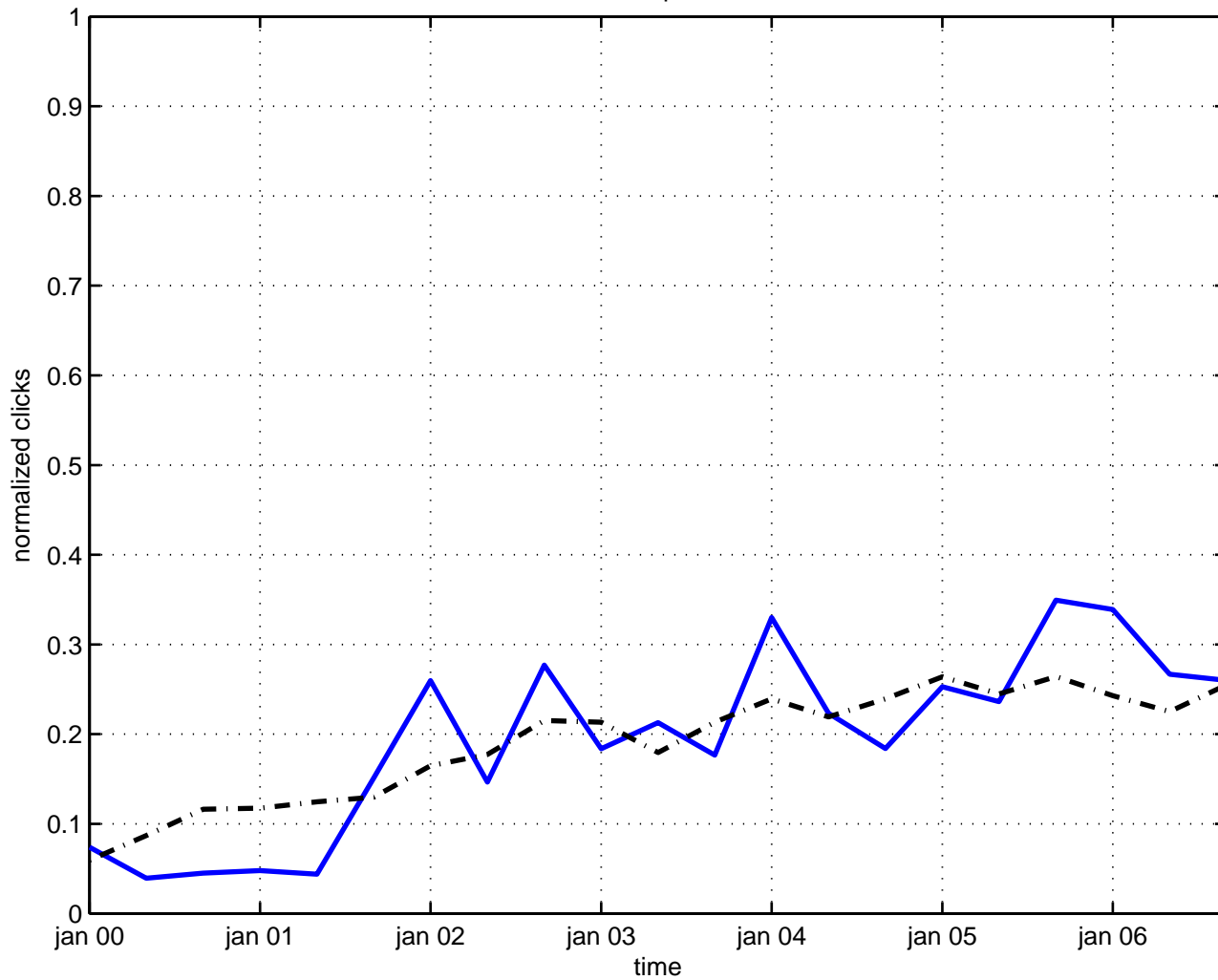
dirac equation
