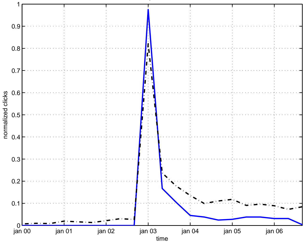
dipole model
